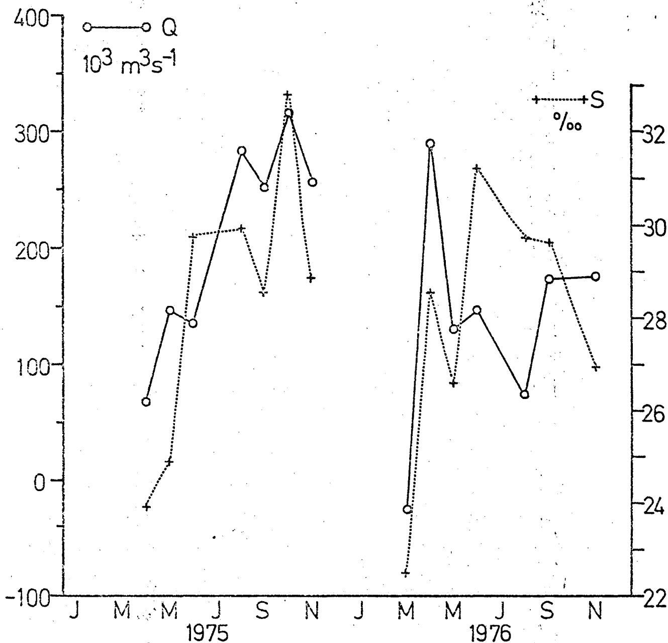
Fig. 3. Mean geostrophic volume transport (Q) and surface salinity (S)
